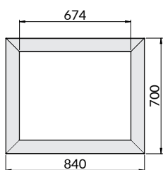
Aro / Marco / Frame 83 mm
