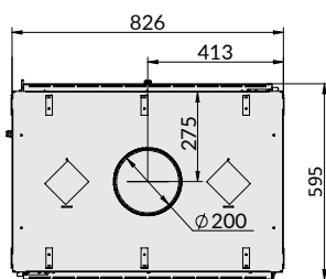
Vista topo Vista superior / Top view
