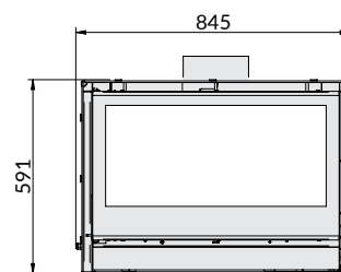
Vista frontal Vista frontal / Front view
