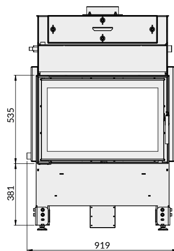
Vista frontal Vista frontal Front view
